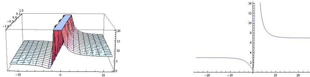
Figure 4: The solution (46) is shown at the above two or three dimensional graphs for the values \tau_0 = \tau_1 = \tau_2 = \alpha_1 = a = b = 1 , \alpha_2 = 2 , n = -1 , t = 1 .
