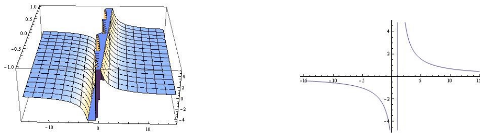
Figure 1: The solution (29) is shown at the above two or three dimensional graphs for the values \tau_0 = a = b = -1 , \tau_1 = \alpha_1 = \zeta_1 = \zeta_2 = 1 , n = -2 , t = 1 .
