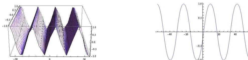
Figure 3: The solution (32) is shown at the above two or three dimensional graphs for the values \tau_0 = a = b = -1 , \tau_1 = \alpha_3 = \zeta_1 = \zeta_2 = 1 , \alpha_1 = 3 , \alpha_2 = 2 , n = -2 , t = 1 .
