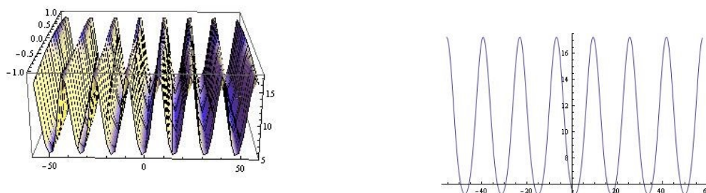
Figure 6: The solution (48) is shown at the above two or three dimensional graphs for the values \tau_0 = \tau_2 = \alpha_1 = a = b = 1 , \alpha_2 = \frac{1}{2} , \alpha_3 = 3 , \tau_1 = \alpha_4 = 2 , n = -1 , t = 1 .
