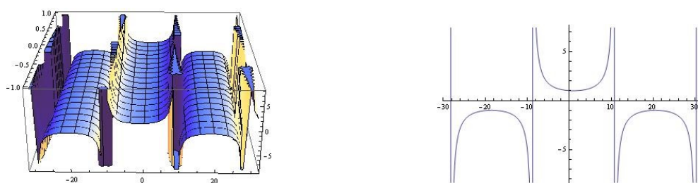
Figure 2: The solution (30) is shown at the above two or three dimensional graphs for the values \tau_0 = a = b = -1 , \tau_1 = \alpha_1 = \zeta_1 = \zeta_2 = 1 , \alpha_2 = 2 , n = -2 , t = 1 .
